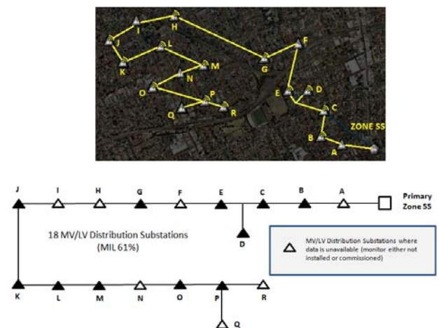
Figure 5 - Sample Feeder Configuration.
