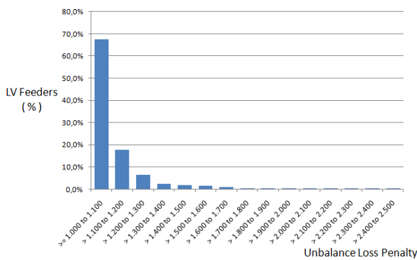
Figure 4 - Distribution of number of feeders in percent with different loss penalties due to unbalance.
